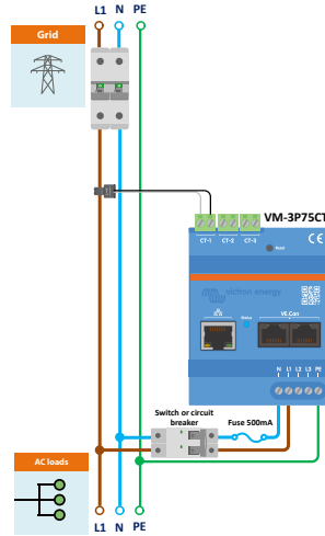
VM-3P75CT 1-phase wiring when used as a grid meter
