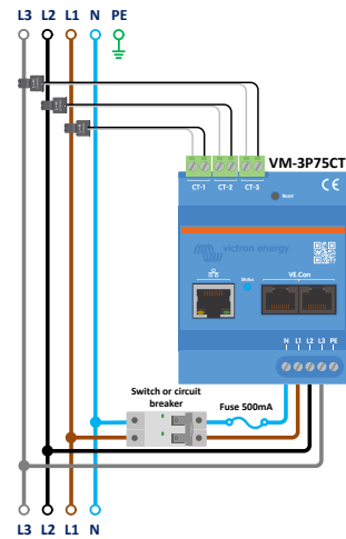
VM-3P75CT 3-phase IT system wiring
