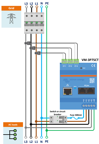
VM-3P75CT 3-phase wiring when used as a grid meter
