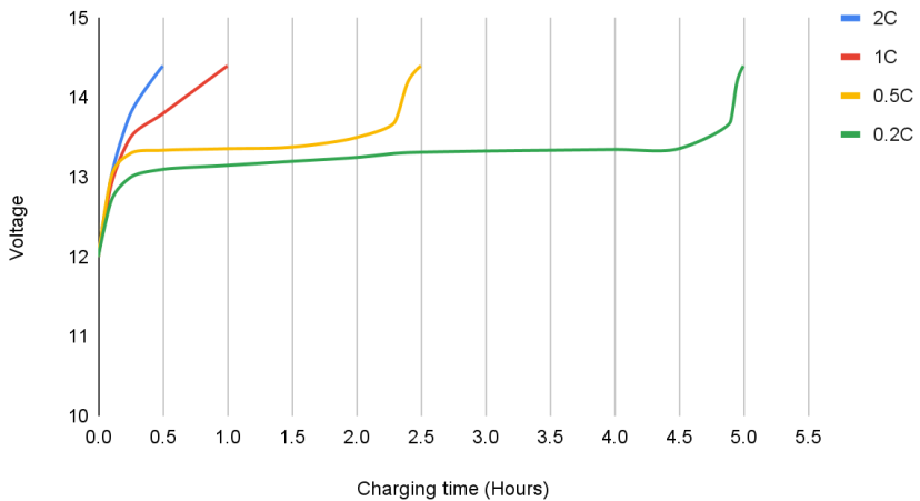
Charging characteristics at different rates
