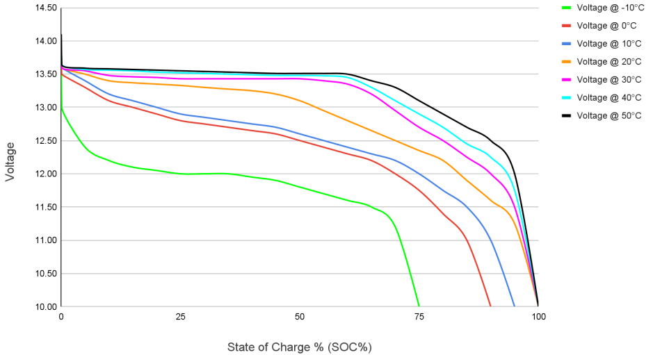
Temperature effect on discharging (0.5C)
