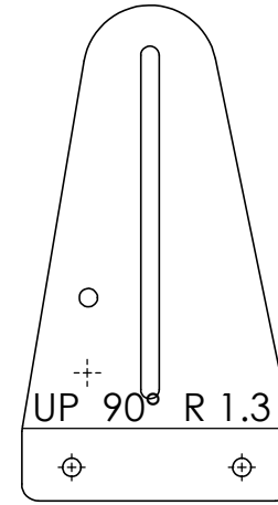
FLAT PATTERN
